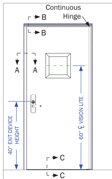
Wet-Side Elevation
