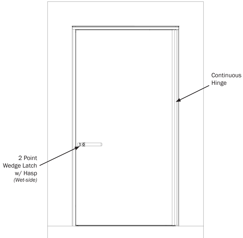
WET-SIDE VIEW (RHR Swing Shown)
