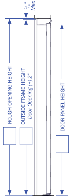
SIDE VIEW
