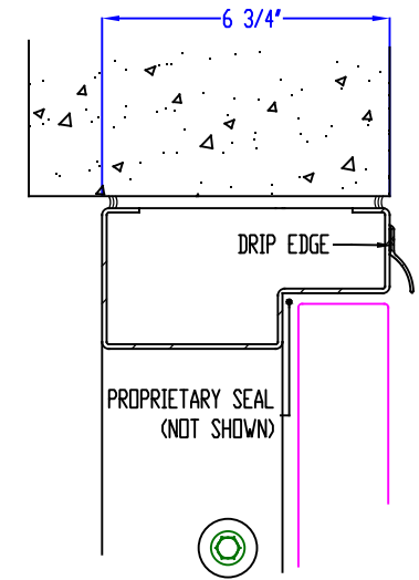
DETAIL E HEAD DETAIL ②④
