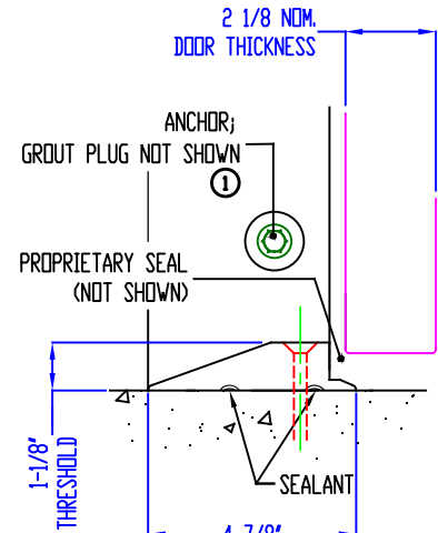
DETAIL F SILL DETAIL
