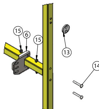
DETAIL E
