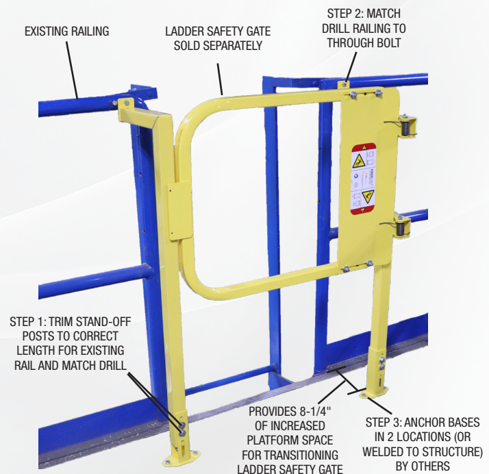
Optional Stand-Off Mounting System shown with Ladder Safety Gate
