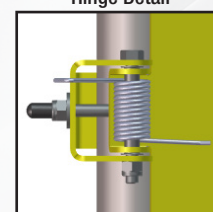
Hinge Detail
