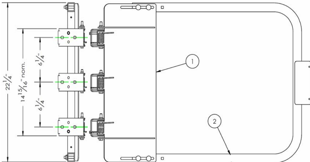
Elevation View
