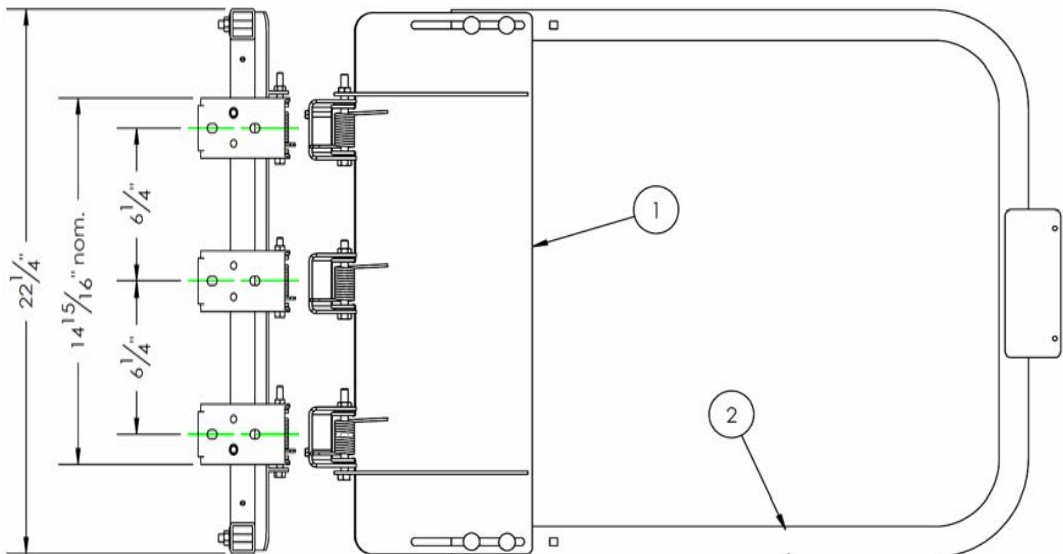
Elevation View
