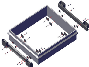
Anchor curb assembly
