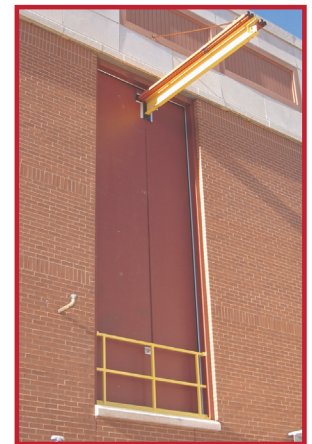
Paired Swing Door for an elevated monorail opening (6'x18')
