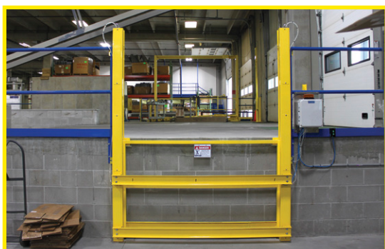
SAFEMEZZ® Downward Gate (MGD)
